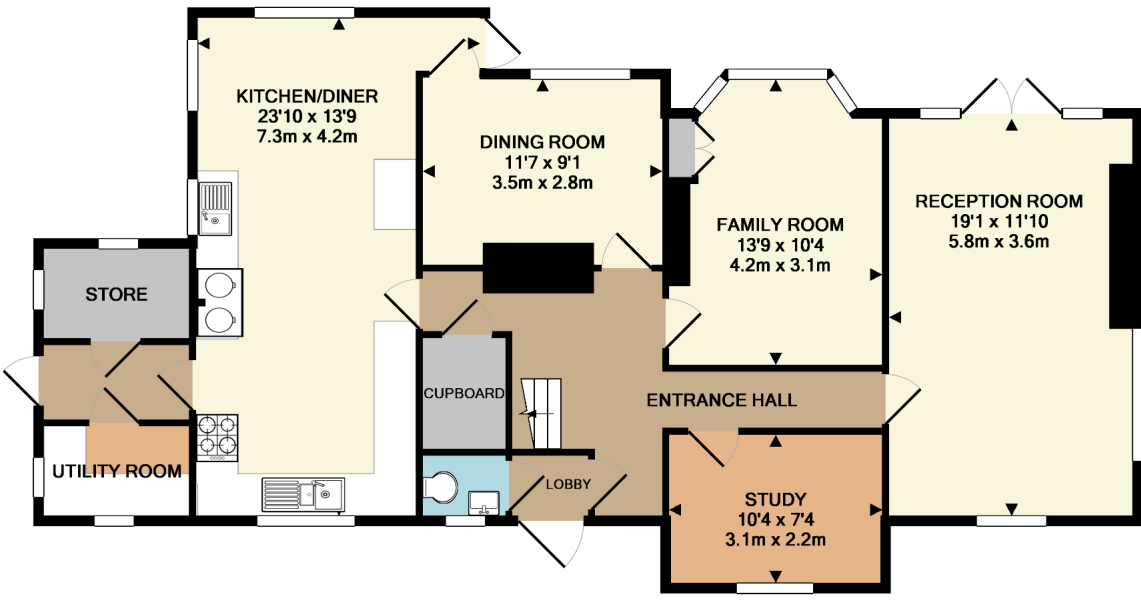
GROUND FLOOR APPROX. FLOOR AREA 1035 SQ.FT. (96.2 SQ.M.)
