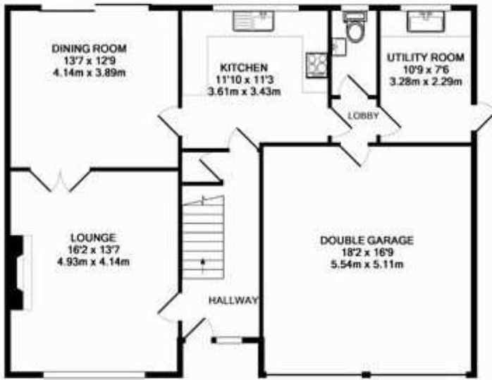
GROUND FLOOR APPROX. FLOOR AREA 97.1 SQ.M. (1045 SQ.FT.)
